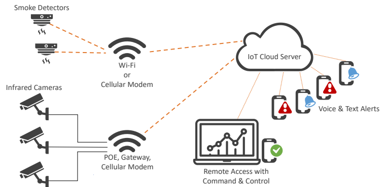
Example MoviTHERM iEFD configuration for Industrial Laundry
