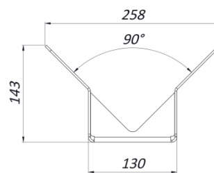
SSCM129 FRONT VIEW
