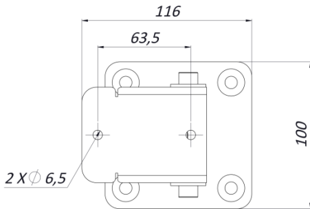
SSPTM129 SIDE VIEW
