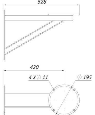
SSBK250 SIDE VIEW
